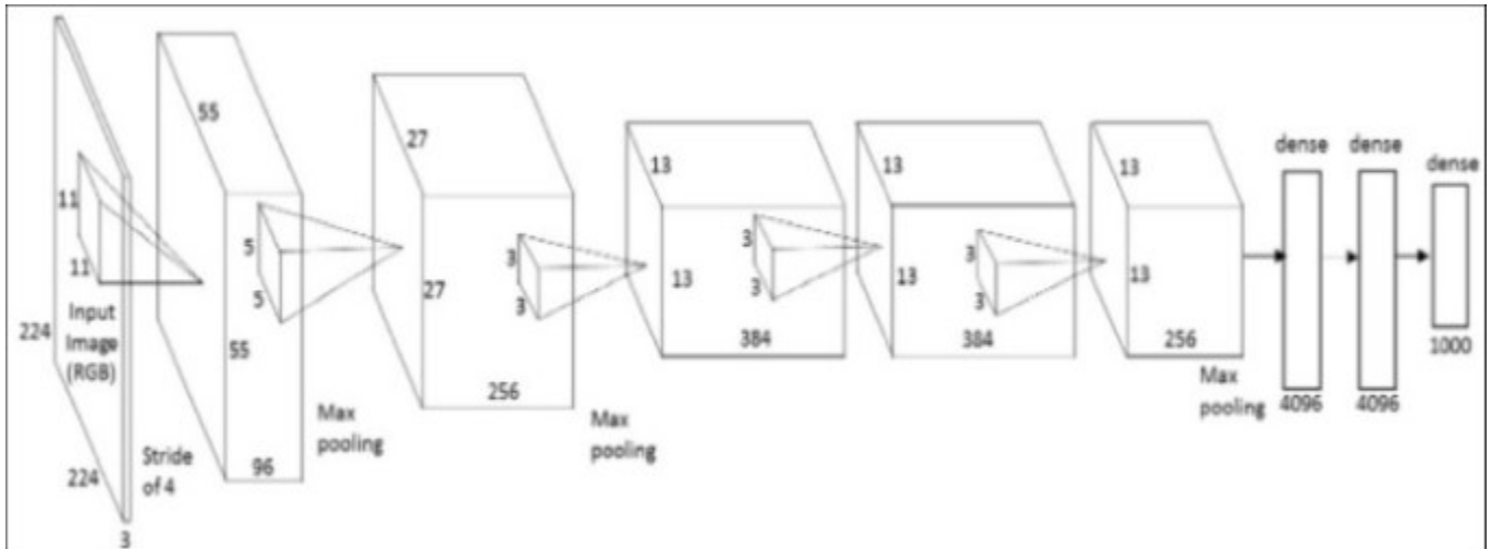
AlexNet architecture
