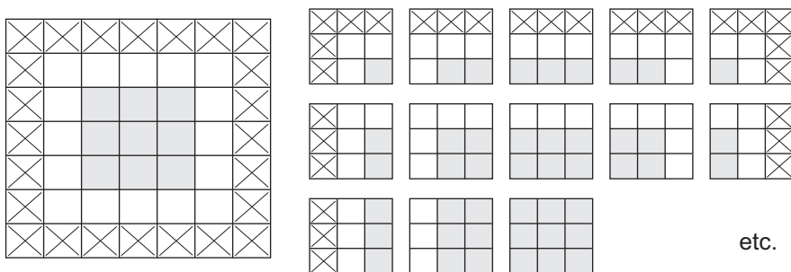
Figure 5.6 Padding a 5 \times 5 input in order to be able to extract 25 \times 3 patches
